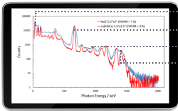
Figure: comparison between LaBr 3 (Ce) and NaI(Tl) detectors sensitivity to identify nuclides
